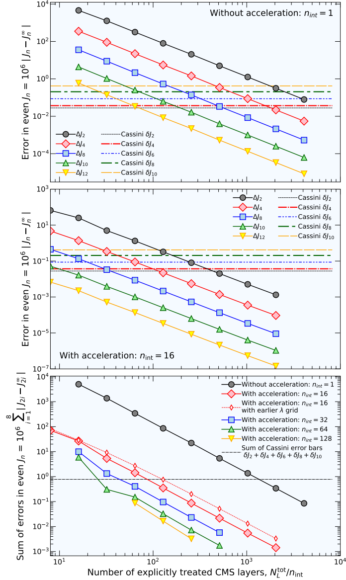
Figure 6. Discretization error of the gravity harmonics calculated with the CMS method as a function of the number of spheroids. The horizontal lines show the 1\text{-}\sigma uncertainties of the Cassini measurements of the even gravity harmonics, J_n . The top panels show how the errors decay with increasing number of layers for calculations without acceleration. The mid panel displays results obtained with the accelerated CMS method where only one in n_{\text{int}} = 16 layers are treated explicitly. 512 explicit layers (total of 8192) are sufficient to reduced the error in all calculated gravity harmonics below the uncertainties of the observations. Without the acceleration, well over 4000 layers is required for this level of precision, as the top panel shows. The bottom panel compares results derived with different acceleration factors, n_{\text{int}} . For n_{\text{int}} = 16 , the effects of two different \lambda discretization schemes are compared.
