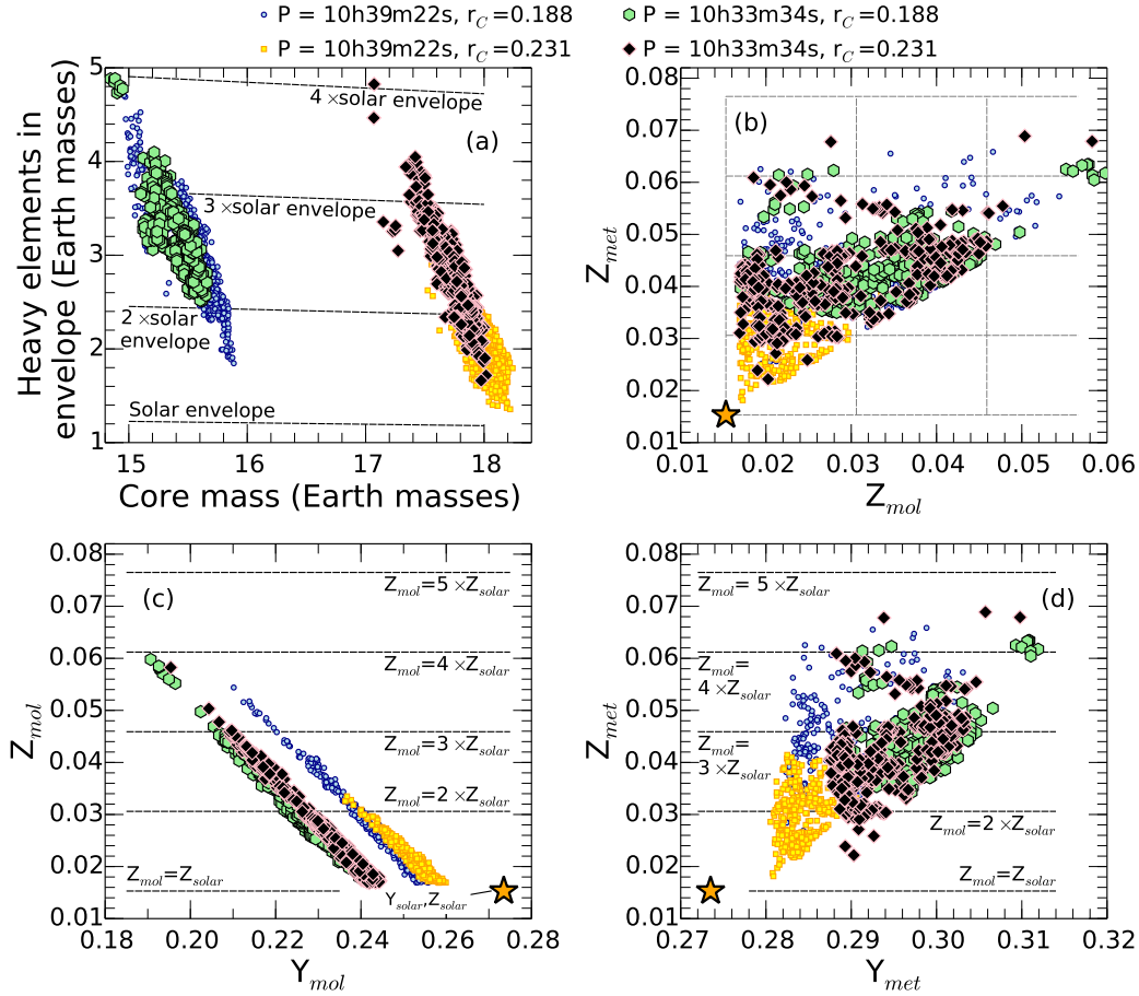
Figure 12. Comparison of parameters from interior models with the preferred rotation rate of 10:33:34 h from this paper, compared to the System III rotation rate (Desch & Kaiser 1981). Core radii r_C = 0.188 and r_C = 0.231 correspond to rocky and rock-ice compositions respectively. (a) The distribution of heavy element mass between the core and envelope. (b) The variation of heavy element mass fraction in the molecular and metallic envelopes. (c) The tradeoff between heavy element and helium mass fractions in the molecular envelope. (d) The tradeoff between heavy element and helium mass fractions in the metallic envelope. In panels (b),(c),and (d) solar values (Lodders 2010) are shown with a yellow star, corresponding solar proportions.
