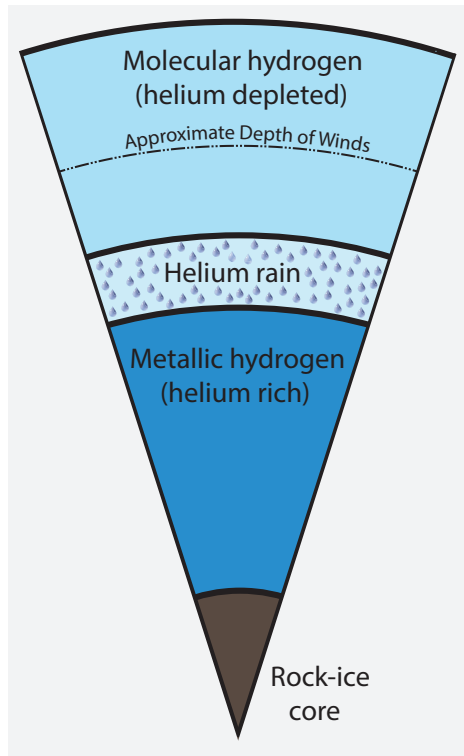
Figure 2. Illustration of the four-layer models for Saturn’s interior that we constructed in this work. We assume an outer molecular and an inner metallic envelope, separated by a helium rain layer, with a dense core at the center of the planet.
