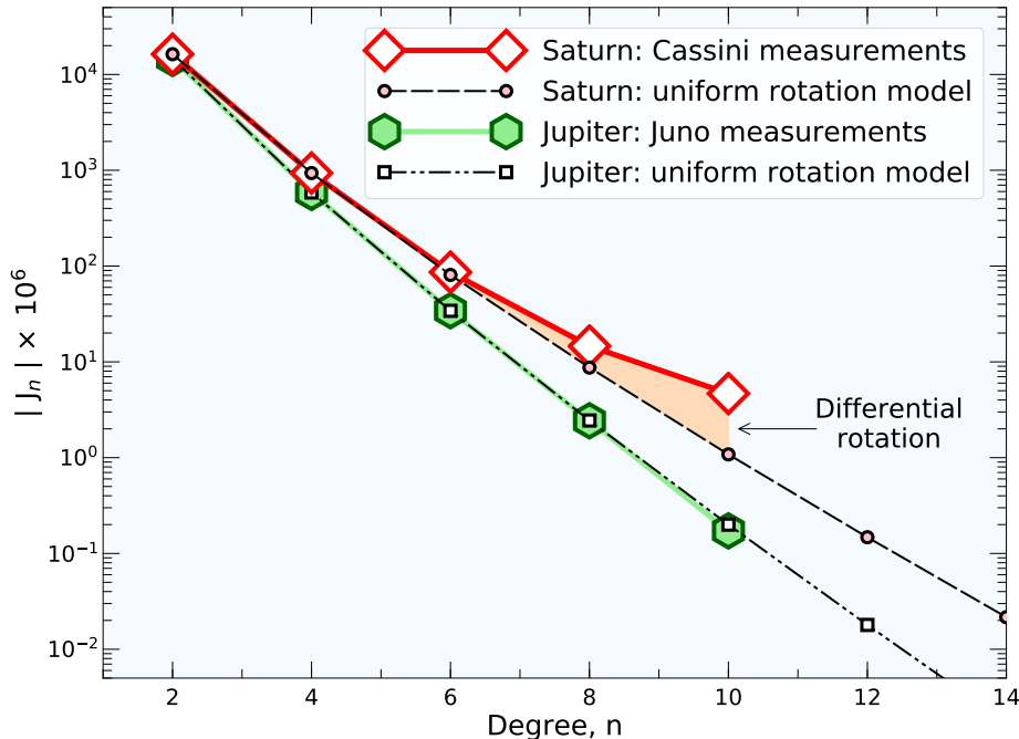
Figure 1. Comparison of the gravity harmonics measured for Jupiter and Saturn with predictions from models assuming uniform rotation throughout the entire interior of both planets. The deviations are small for Jupiter while substantial discrepancies emerge for Saturn. This illustrates that the effects of differential rotation are much more important for Saturn.
