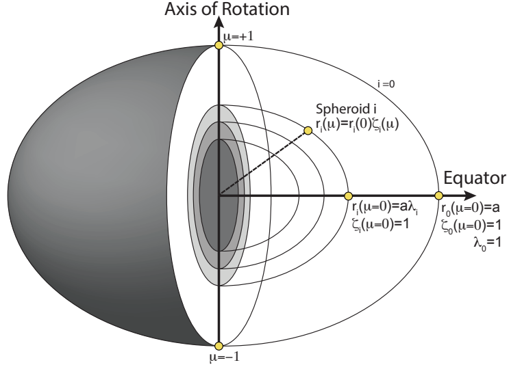
Figure 4. Illustration of the CMS method and variable definitions.
