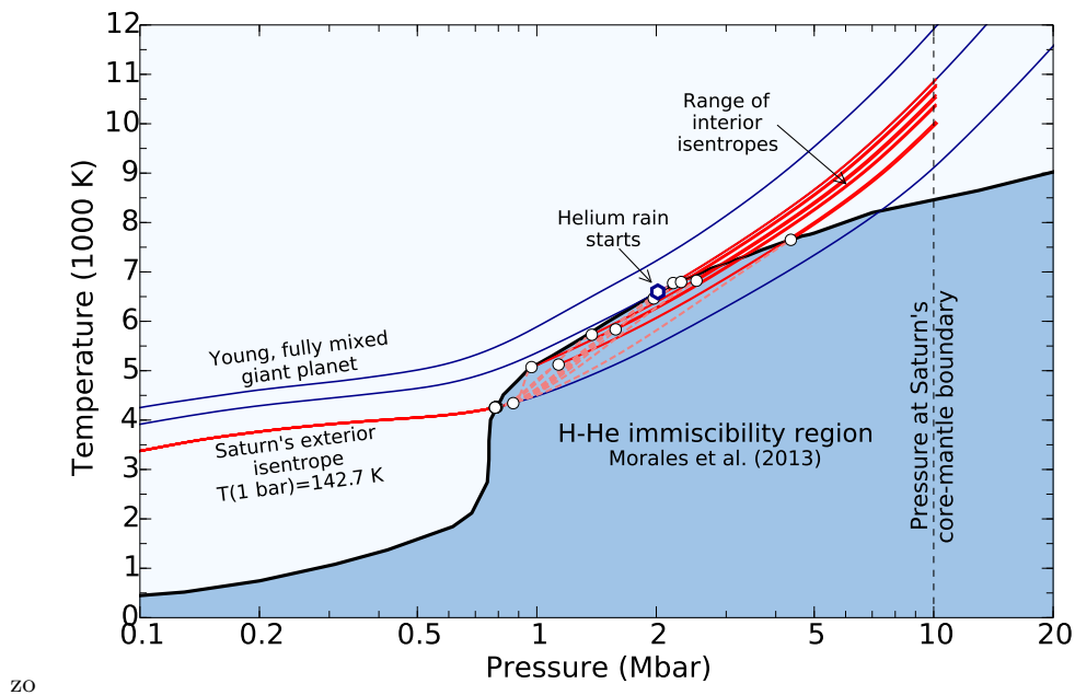
Figure 3. Temperature-pressure phase diagram of hydrogen-helium mixtures. The red lines show the interior models with P=10:39:22 h and r_C=0.2 in relation to the shaded region where the two fluids are predicted to become immiscible (Morales et al. 2013). The thin blue lines show various adiabats of an H-He mixture for a helium mass fraction of Y=0.245 (Lodders 2003). The circles mark the beginning and the end of the immiscibility regions assumed in different models.
