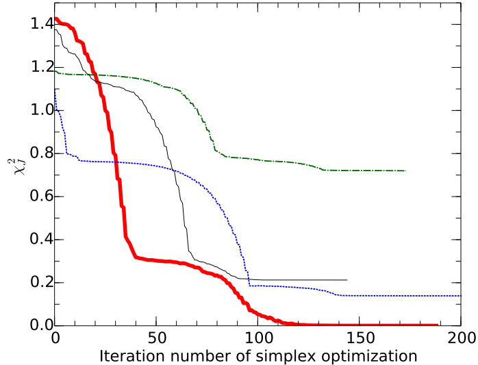
Figure 9. \chi^2_J deviations (see Eq. 27) between the calculated and the observed gravity harmonics during the model optimization with the simplex algorithm. Only one model optimization (thick solid line) succeeded in converging to a state that matched the spacecraft measurements well.
