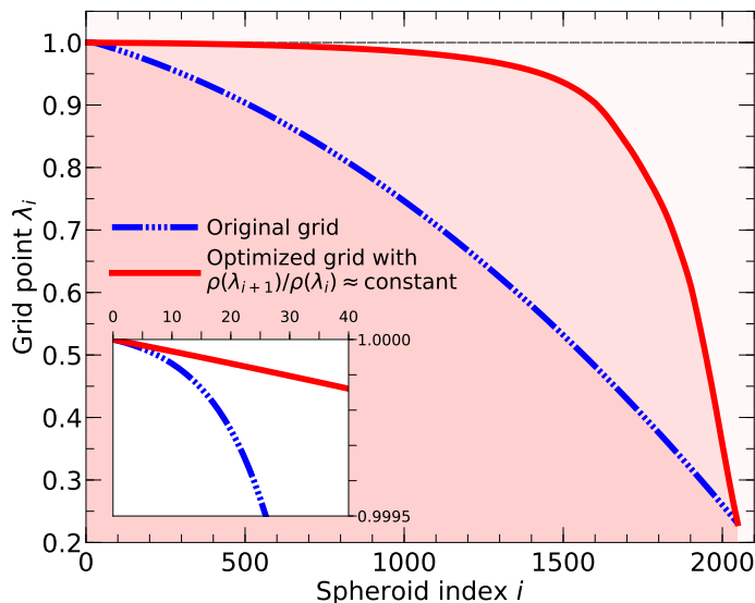
Figure 7. Comparison of our original and optimized \lambda grids for an interior model with 2049 spheroids and r_C=0.231 .
