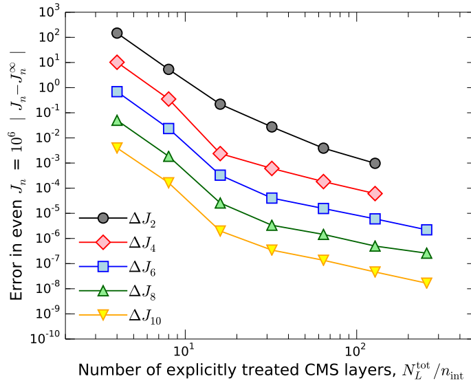
Figure 8. Discretization error in the gravity harmonics of polytrope index 1 planet models. The error of all gravity harmonics decays with increasing spheroid number, as we have seen for the Saturn interior models in Fig. 6. All calculations for this figure were performed with n_{\text{int}} = 256 .
